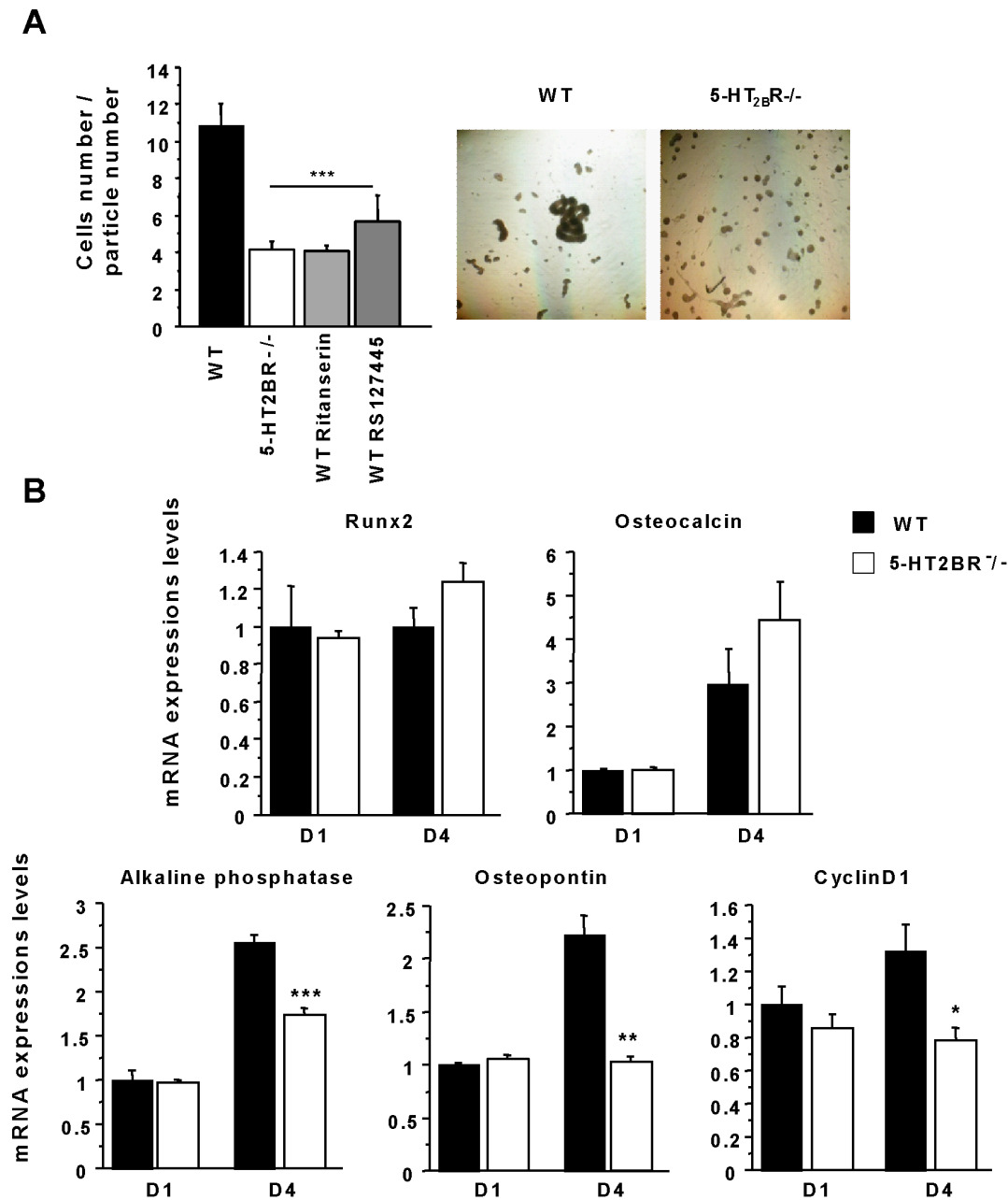
Figure 1. Cell-cell adhesion and expression profile of osteoblastic markers of 5-HT 2B R -/- osteoblasts. A: Representative pictures of aggregation assays are shown at Day 1 (D1) after the induction of 5-HT 2B R -/- and WT primary cultures. Counts of cell aggregates were assessed in WT, and 5-HT 2B R -/- cells, and in WT cells treated with either ritanserine (an inverse agonist of 5-HT 2 R) or RS127445 (a selective 5-HT 2B R antagonist). The 5-HT 2B R -/- and WT-treated cells displayed a much lower level of cell adhesion than the untreated WT cells. B: the main markers of osteoblast differentiation were measured by RTqPCR. Runx2, osteocalcin expression levels were not modified by the absence of 5-HT 2B R, whereas cyclin D1, alkaline phosphatase and osteopontin expression levels were decreased. Data are presented as means \pm SEM of three independent experiments performed in triplicate. ** p < 0.005 vs WT, * p < 0.05 vs WT. doi:10.1371/journal.pone.0075783.g001
