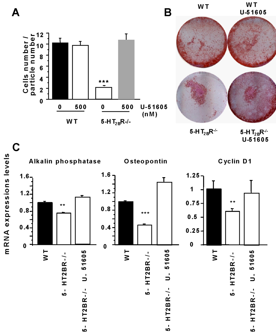
Figure 3. 5-HT 2B R -/- osteoblasts phenotype is dependent on prostacyclin overexpression. A specific inhibitor of prostacyclin synthase (U51605) was used to evaluate the role of the prostacyclin overproduction. A: a cell aggregation assay was performed with this inhibitor on WT and 5-HT 2B R -/- cells. U51605 had no effect on WT aggregation and restored 5-HT 2B R -/- cell aggregation. B: mineralization assay: U51605 had no effect on WT cells, but did rescue 5-HT 2B R -/- mineralization. C: The expressions of the alkaline phosphatase, osteopontin and cyclin D1 level markers modified by the absence of 5-HT 2B R were restored by adding U51605 to 5-HT 2B R -/- osteoblasts. Data are presented as means \pm SEM of three independent experiments performed in triplicate. ** p < 0.05 vs. WT, *** p < 0.001 vs. WT. §§§ p < 0.005 vs 5-HT 2B R -/- . doi:10.1371/journal.pone.0075783.g003
