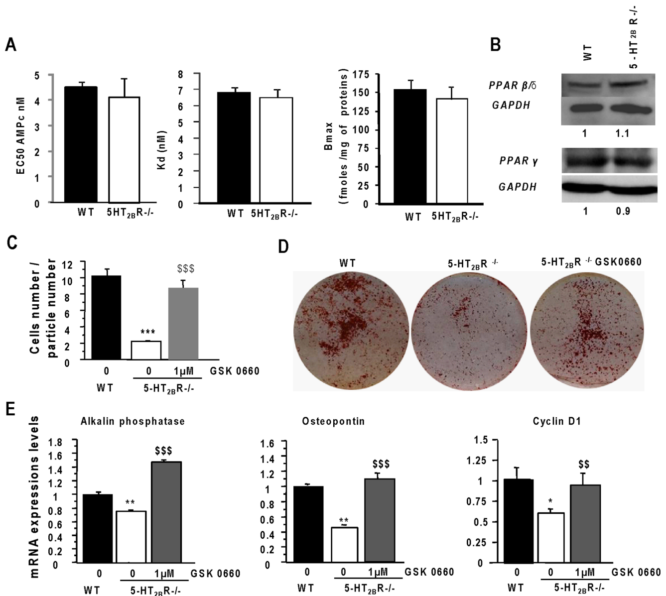
Figure 4. Pharmacological inhibition of PPAR- \beta/\delta restores the phenotype of 5-HT 2B R -/- osteoblasts. PGI 2 is an endogenous ligand of nuclear PPAR \beta/\delta , and also can act via the membrane IP receptor. We evaluated the involvement of these two potential prostacyclin targets in 5-HT 2B R -/- cells. A: For the membrane IP receptor: the cAMP level and the binding parameters of the IP receptors were measured in both cell types. None of these parameters was modified by the absence of the 5-HT 2B receptor. B: PPAR- \beta/\delta and PPAR- \gamma expressions were analyzed by Western blotting, and found to be unchanged in both cell types. The involvement of PPAR \beta/\delta was determined using specific antagonist of this receptor. C: An aggregation assay was carried out in the presence of GSK0660 (a specific antagonist of PPAR- \beta/\delta ) for 5-HT 2B R -/- cultures. The GSK0660 treatment restored cell aggregation in 5-HT 2B R -/- cultures. D: A mineralization assay (red alizarin staining) was performed under the various different conditions: GSK0660 treatment rescued the phenotype in 5-HT 2B R -/- osteoblasts. E: Similar results were obtained for the transcriptional expressions of the alkaline phosphatase, osteopontin, and cyclin D1 level markers. Data are presented as means \pm SEM of three independent experiments performed in triplicate. *** p < 0.005 vs. WT and $$$ p < 0.005 vs 5-HT 2B R -/- . doi:10.1371/journal.pone.0075783.g004
