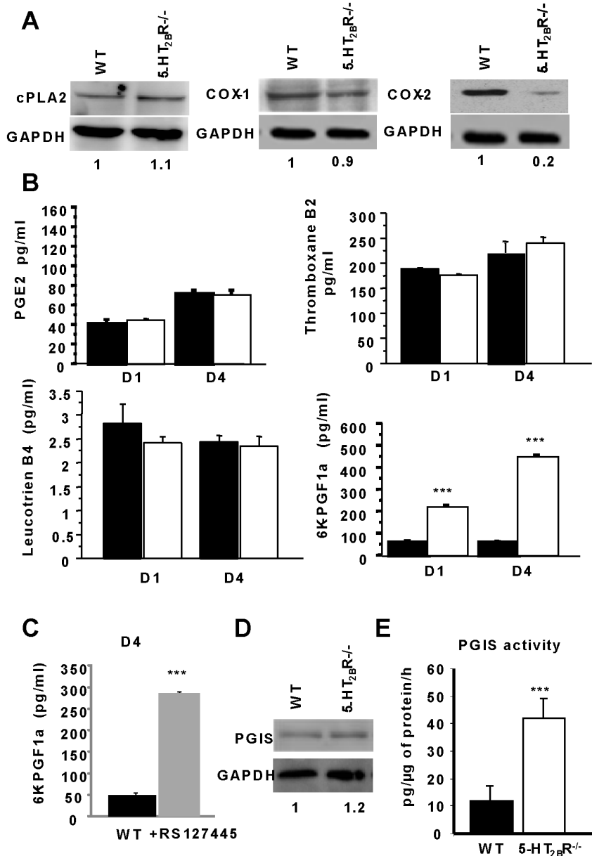
Figure 2. Prostacyclin over-produced in 5-HT 2B R -/- osteoblasts. A: To determine the role of the PLA 2 pathway in the 5-HT 2B R -/- osteoblasts, the expression of PLA 2 and of COX 1 and COX 2 were analyzed by Western blotting. The expression of COX 2 was markedly lower in the 5-HT 2B R -/- cells than in the WT cells, whereas no difference was observed in the expression of PLA 2 or COX 1 . B: Measurement of the main eicosanoids in both genotypes: Prostaglandin E 2 , Thromboxane B 2 , Leukotriene B 4 and 6-keto prostaglandin F 1 α, a stable metabolite of prostacyclin, at D1 and D4. Prostacyclin production was greater in 5-HT 2B R -/- primary cultures than in WT cultures. C: It was also greater in WT cultures treated with RS 127445 at D4. D: Prostacyclin synthase expression was evaluated by Western blotting. Levels of prostacyclin synthase were slightly higher in 5-HT 2B R -/- than in WT cultures. E: Prostacyclin synthase activity was markedly higher in 5-HT 2B R -/- than WT cultures. Data are presented as means ± SEM of three experiments performed in triplicate. *** p<0.001 vs. WT. doi:10.1371/journal.pone.0075783.g002
