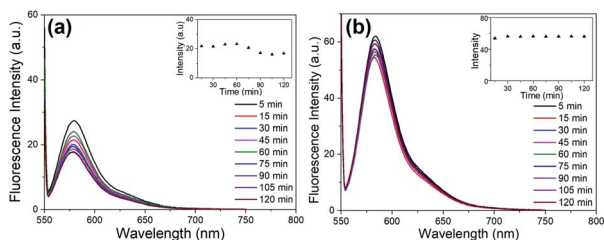
Fig. 6 Fluorescence spectra of FSNP-APTES (10%) (a) and FSNP-EDC/NHS (4 : 1) (b) over 120 minutes with an increment of 15 minutes. The inset shows the fluorescence intensity at 588 nm over 120 minutes.
