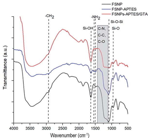
Fig. 2 FTIR spectra of the fluorescent silica nanoparticles, FSNPs (black), FSNPs after silanization, FSNP-APTES (blue), and silanized FSNPs after reaction with glutaraldehyde, FSNP-APTES-GTA (red).
