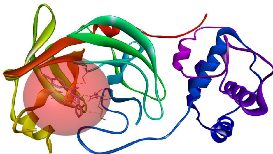
Fig. 9. Main protease (6LU7) with CCPEHP inhibitor.
