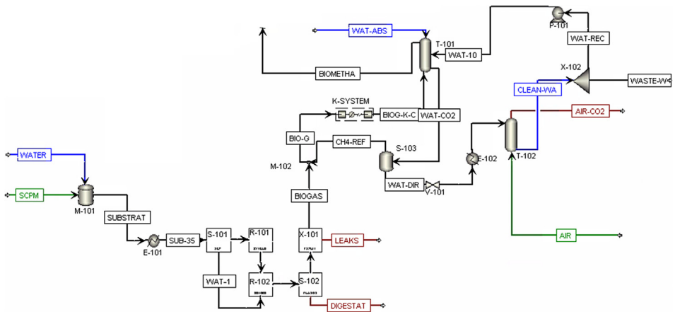
Fig. 5. Aspen flowsheet for the simulation of biomethane using sugarcane press-mud. E: Heat exchanger; S: Separator; M: Mixer; X: Component splitter; T: Absorption/Stripping towers; P: pumps; K: Compressor system.
