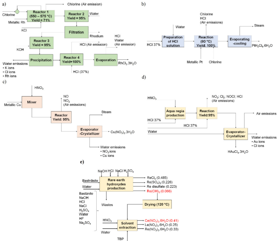
Fig. 8. Block flow diagram to produce a) RhCl 3 ·3H 2 O; b) PtH 2 Cl 6 ·6H 2 O; c) Cu(NO 3 ) 2 ·3H 2 O; d) HAuCl 4 ·3H 2 O; e) Ce(NO 3 ) 3 ·6H 2 O. Values in parenthesis are mass allocation factors.
