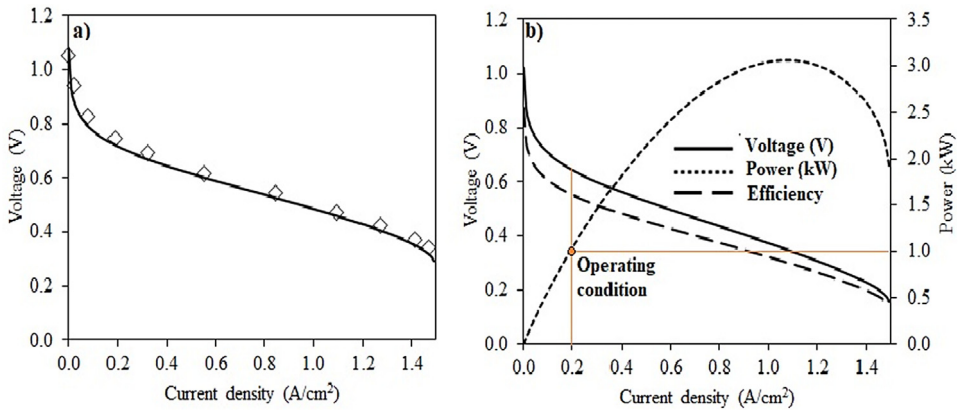
Fig. 4. a) Validation of a Ballard Mark V fuel cell. Continuous line: Aspen model; \diamond Experimental data. Fuel cell parameters: T = 343 K, P = 1 atm, P_{H_2} = 1 atm; P_{O_2} = 1 atm; A = 50.6 cm 2 ; and n = 1 . b) Fuel cell performance at the operating conditions of the power production plant. T = 348 K, P = 0.81 atm.
