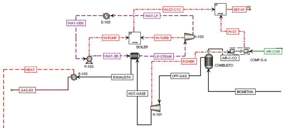
Fig. 6. Aspen flowsheet to produce power and heat from bi methane by using a Rankine cycle.
