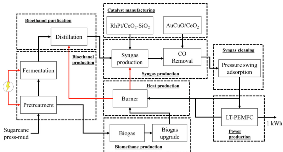
Fig. 1. Foreground system to produce power from sugarcane press-mud.
