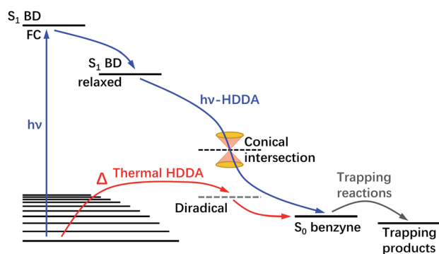
Fig. 7 Schematic illustration of the mechanism of the photochemical ( h\nu ) and thermal HDDDA reactions. The h\nu -HDDA mechanism (blue path) is revealed by the present work, while the thermal HDDDA mechanism was reported by Wang et al. 26 and included here for comparison.
