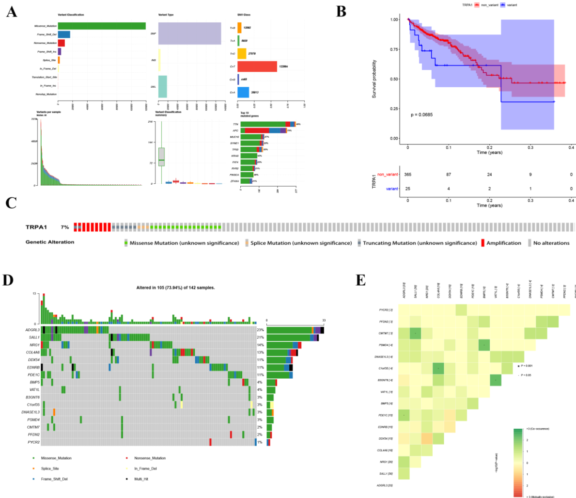
Fig. 4: TRPA1 and mutations in COAD samples. A. Summary of mutation information in COAD samples. B. K-M survival curves of patients with mutated and non-mutated TRPA1 . C. Mutations of TRPA1 gene in COAD samples. D. Waterfall plot to display the mutations in 16 TRPA1 -related genes in COAD samples. E. The correlation analysis of 16 TRPA1 -related mutant genes
