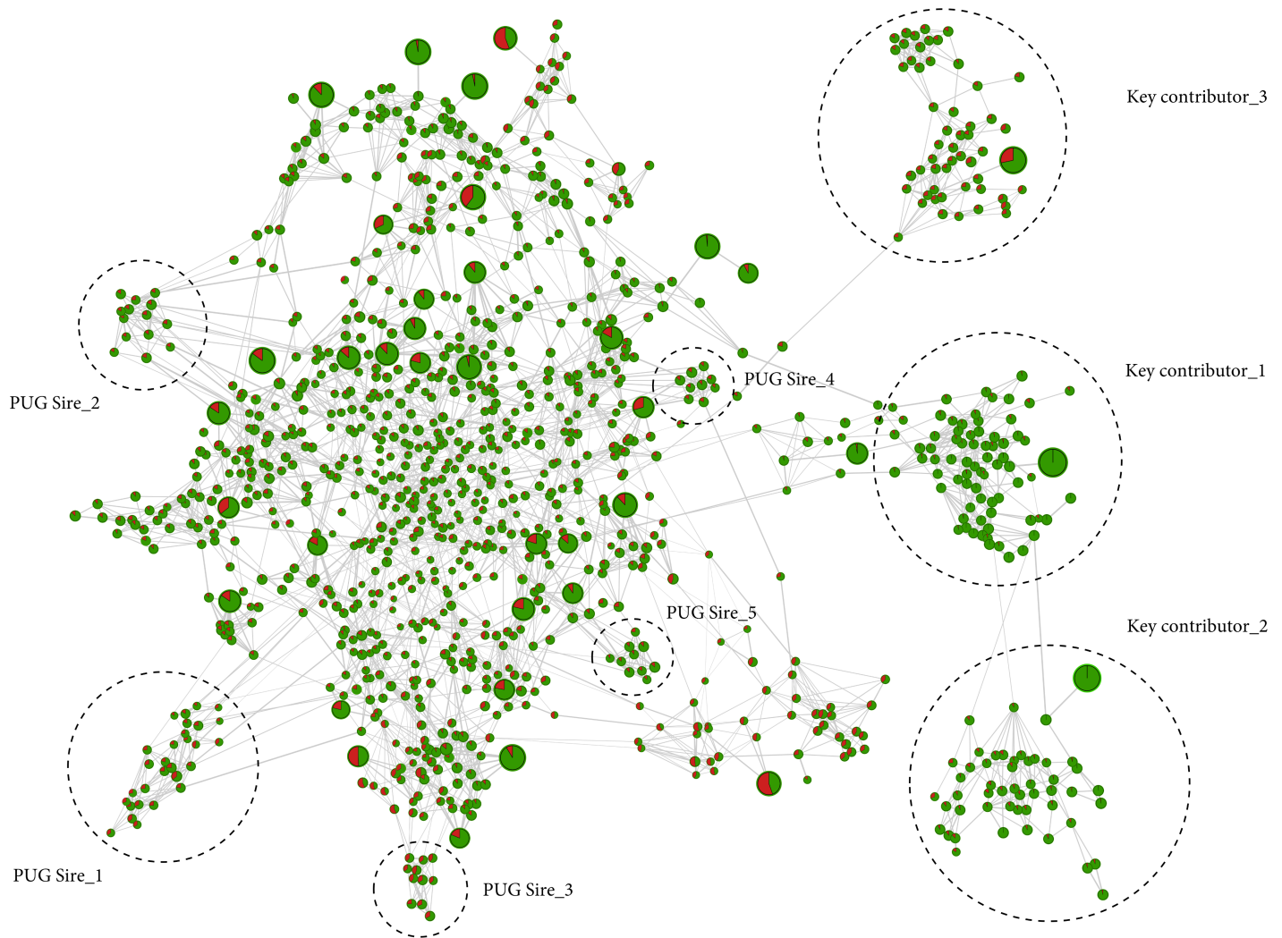
Fig 5. High-resolution population structure of horse. Network visualization of 1,077 horses. Each horse is represented by a node; with individual node size associated with g_c , whilst the two different node colors represent a_j between Swiss Franches-Montagnes (FM) (green) and Warmblood (red). Top 41 key contributors are represented by an increased node size. The thickness of edges varies in proportion to the genetic distance to visualize individual relationships within the population. The topology of the network reflects the population structure of the FM horse breed and reveals sub-structures caused by the progeny of most influential stallions. The progeny clusters of the three most influential stallions and un-genotyped sires (PUG) are indicated by a dashed circles.
