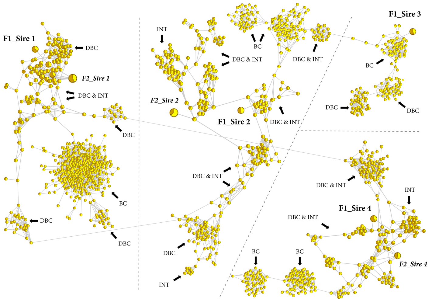
Fig 4. High-resolution population structure of experimental sheep. Network visualization of 1,421 sheep. Each sheep is represented by a node; with individual node size associated with gc_j , whilst the different node colors represent a_j between Awassi (brown) and Merino (yellow). Top seven key contributors are represented by an increased node size. The thickness of edges varies in proportion to the genetic distance to visualize individual relationships within the population. The progeny of the four different F1 sires are separated by dashed lines, whilst the different progeny cluster: backcross (BC), double backcross (DBC) and intercross (INT) are denoted by an arrow.
