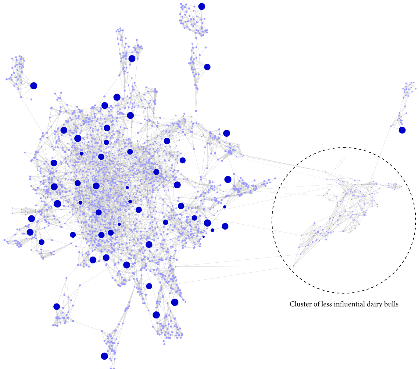
Fig 6. High-resolution population structure of cattle. Network visualization of 2,457 cattle. Each cattle is represented by a node; with individual node size associated with gc_j , whilst the node color (dark blue) indicates top 55 key contributors. The thickness of edges varies in proportion to the genetic distance to visualize individual relationships within the population. The network structure of indicates that key contributors are well distributed within the population and highlights the existence of a substructure according to less influential bulls (dashed circle).
