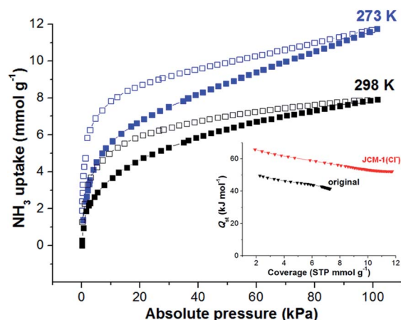
Fig. 5 \text{NH}_3 adsorption isotherms of JCM-1(Cl - ) at 273 K and 298 K. Inset: isosteric heat of sorption ( Q_{st} ) of \text{NH}_3 in JCM-1 and JCM-1(Cl - ) .
