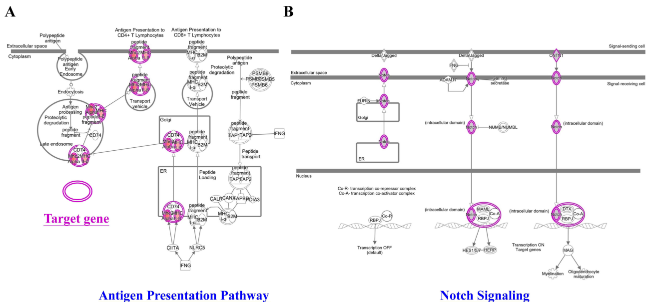
Figure 5 Network analyses of the antigen presentation pathway target gene (A) and the gene that Notch signaling targets (B). IPA software analyzed network analysis (SNPs gene loci, P < 1E-05 ).
