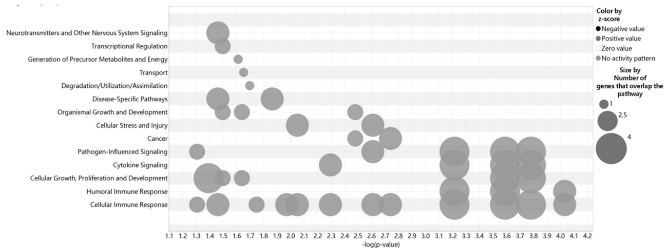
Figure 4 Network studies of 882 SNP gene locations that are associated with AA. Cross analysis of the number of genes and pathways (SNPs gene loci, P < 1E-05 ).
