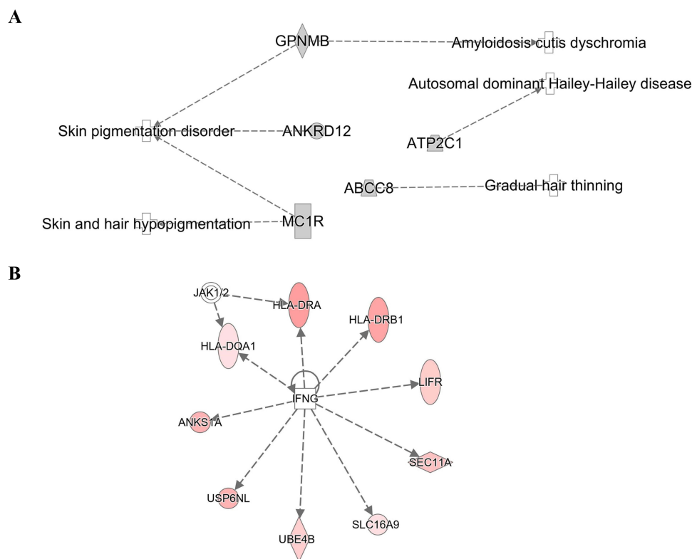
Figure 6 The genetic markers associated with skin and hair diseases ( A ). Nine genetic markers associated with the IFN- \gamma -JAK-STAT signal transmission pathway ( B ). IPA software analyzed network analysis (SNPs gene loci, P < 1 \times 10^{-5} ).
