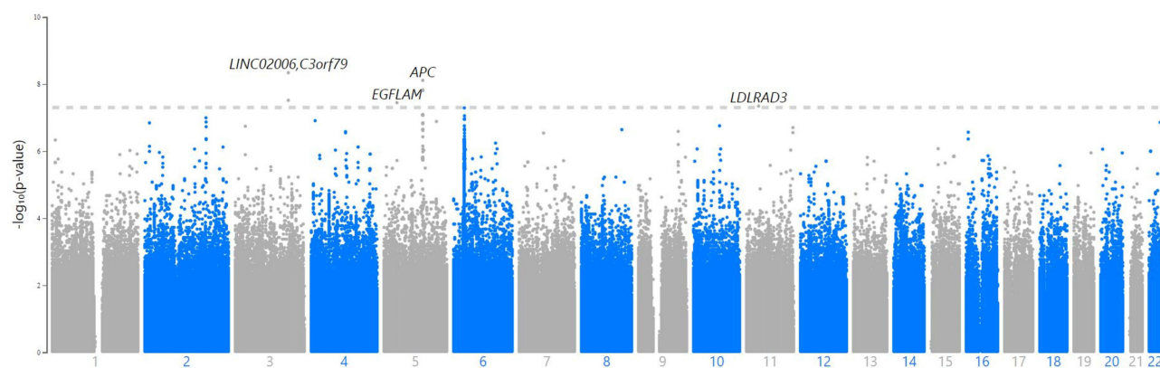
Figure 1 The relationship of genome-wide variations with AA as determined by Manhattan plot analysis. SNP that passed quality control are plotted on the X-axis according to their chromosomal locations versus the Y-axis in Manhattan plot analysis ( -\log_{10} p -value). The higher solid line represents the genome-wide significance criterion ( P < 5E-8 ).
