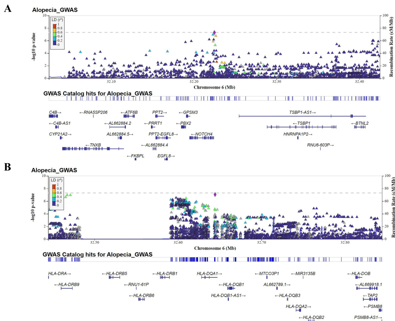
Figure 3 Regional association plot of NOTCH4 (A) and HLA-DQA1 gene (B) in AA. Regional plots for the loci showing significant differences in effect-size estimates. The plot typically shows the position of each SNP along the x-axis and the negative log10 P-value. Color of the point was used to show the linkage disequilibrium (LD) between SNPs.
