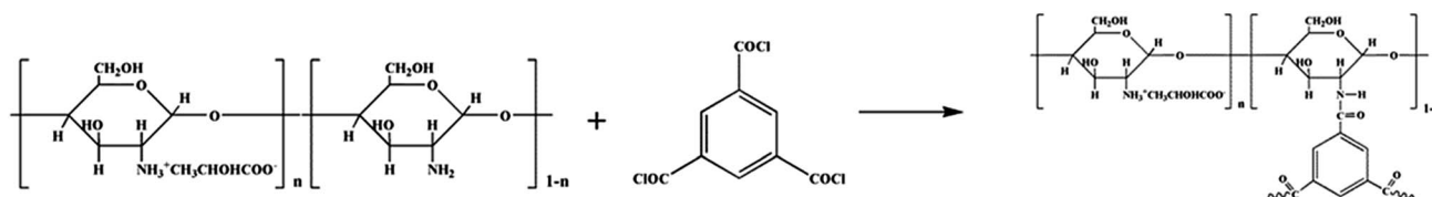
Scheme 1 Interfacial polymerization between CL and TMC.
