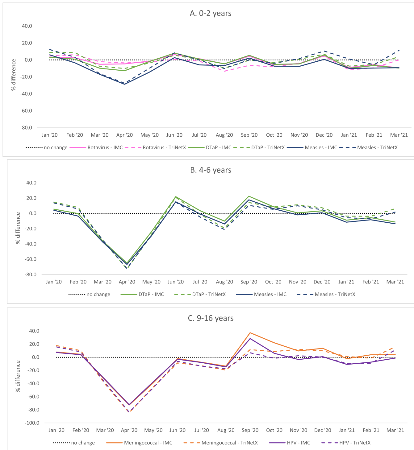
Fig. 3. Percent difference of vaccination administration, 2020 and 2021 vs. 2018–2019 and 2021 vs. 2018–2019, for select vaccines, IBM MarketScan Commercial Database (IMC) with Early View and TriNetX Dataworks: (A) 0–2 years, (B) 4–6 years, (C) 9–16 years.
