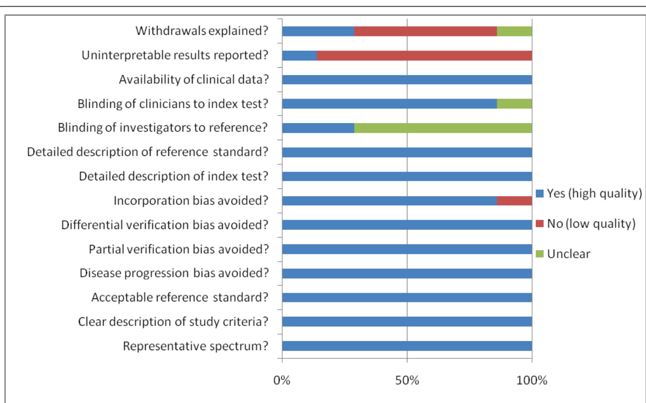
Figure 2 Summary of the methodological quality assessment of the included studies. Bars filled with blue/red/green color indicate the percentage of the studies that meet/do not meet the criteria/do not provide adequate relevant data, respectively.
