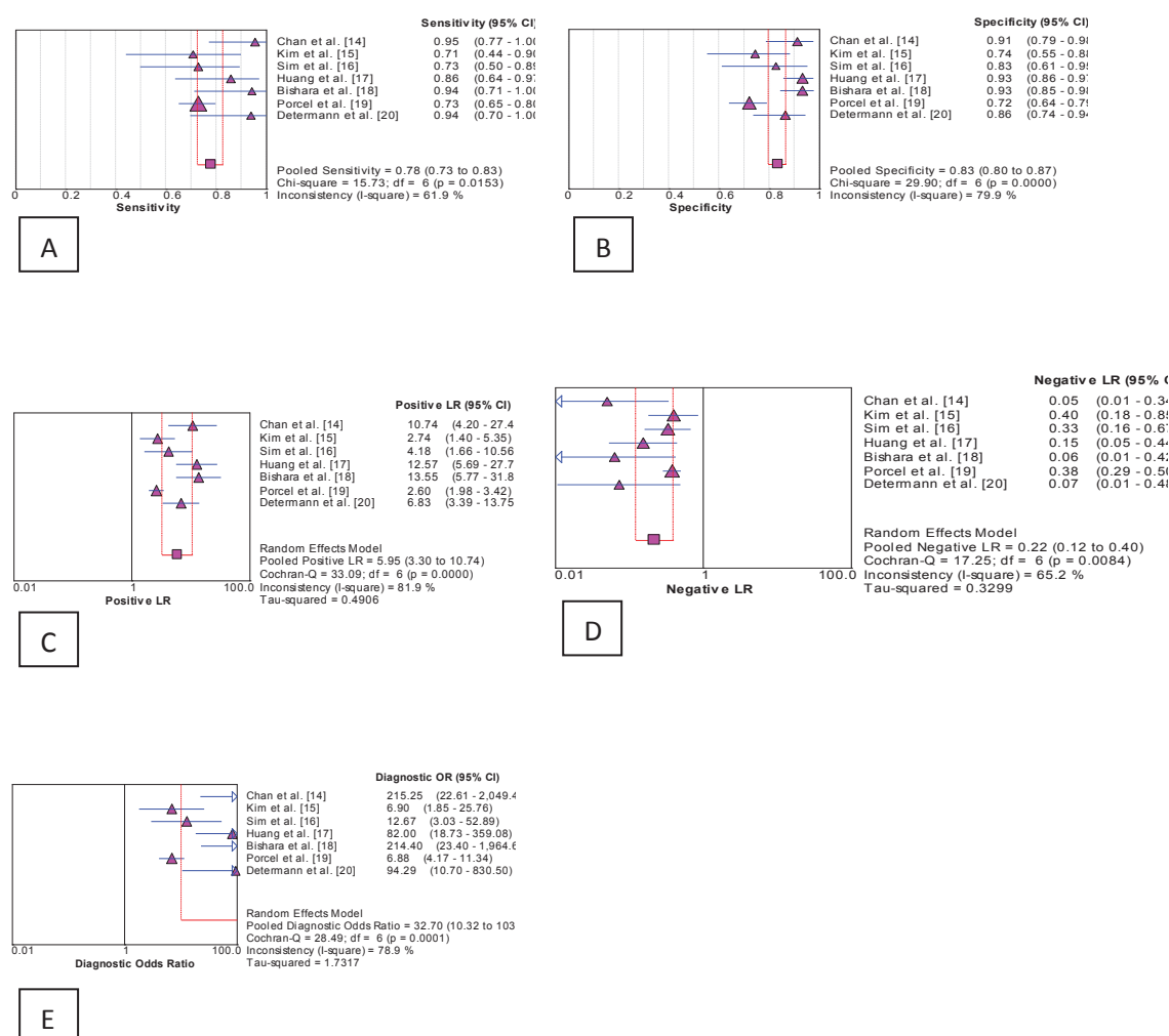
Figure 3 Forest plots of A. sensitivity, B. specificity, C. positive likelihood ratio, D. negative likelihood ratio and E. diagnostic odds ratio of pleural fluid sTREM-1 for the diagnosis of bacterial effusions.
