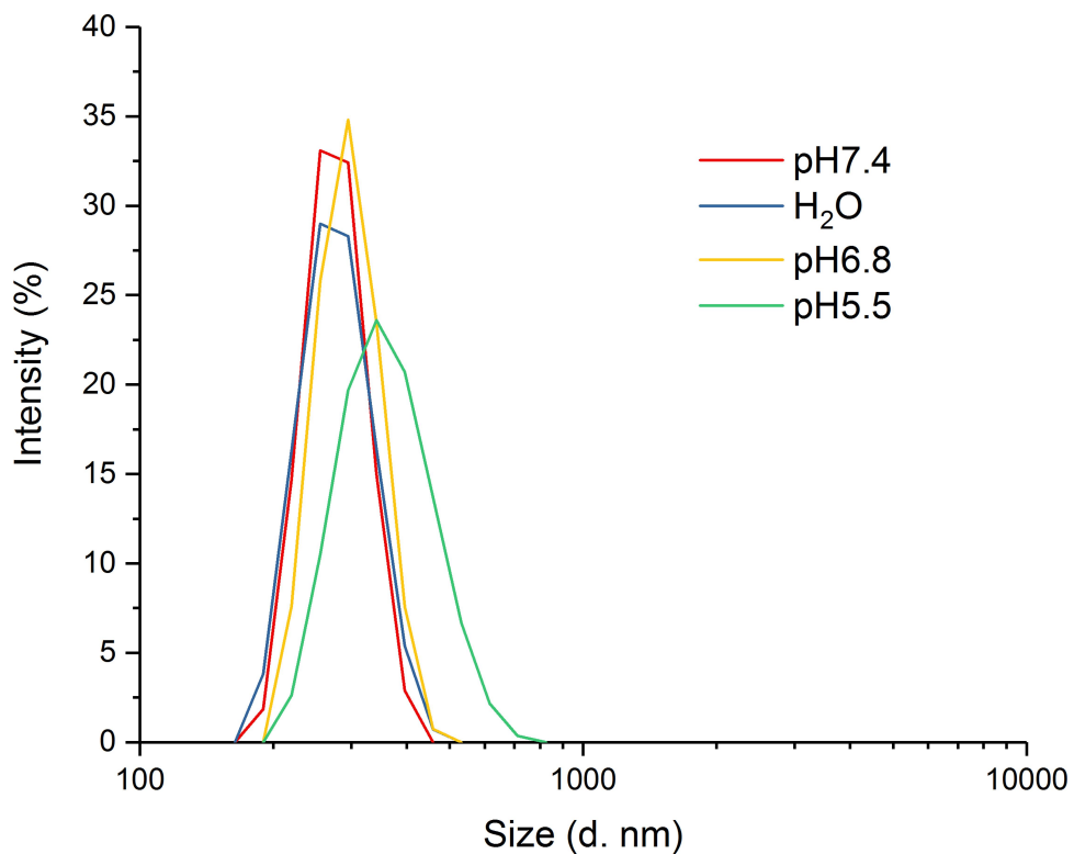
Figure 2 The particle size distribution of the nanogel in H 2 O and PBS solutions (pH 7.4, 6.8 and 5.5).
