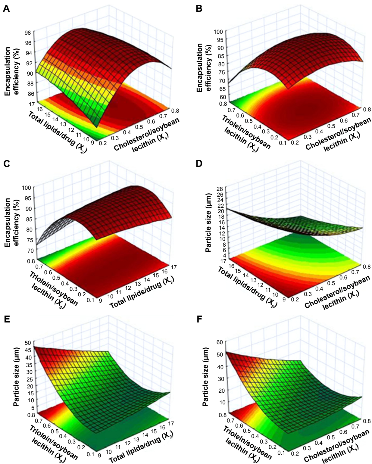
Figure 2 Response surface plot and contour map of the combined effect of (A, D) X_1 and X_2 , (B, F) X_1 and X_3 , and (C, E) X_2 and X_3 on the encapsulation efficiency (%) and the particle size ( \mu\text{m} ).
