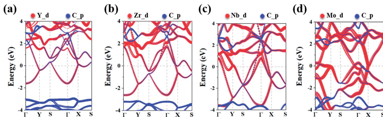
Fig. 3 The electronic band structures of the (a) \text{YC}_2 , (b) \text{ZrC}_2 , (c) \text{NbC}_2 , and (d) \text{MoC}_2 monolayers. The red and blue curves denote the d orbits of the metal atoms and the p orbits of C atoms, respectively. The Fermi energy is denoted by a dashed line at 0 eV.
