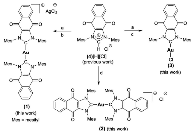
Scheme 1 Preparation of complexes 1–3 from 4[H][Cl]. a = Ag 2 O, CH 2 Cl 2 , b = 0.45 (C 4 H 8 S)AuCl, THF, c = (C 4 H 8 S)AuCl, THF, d = NaN(SiMe 3 ) 2 , toluene, and 0.45 (C 4 H 8 S)AuCl.
