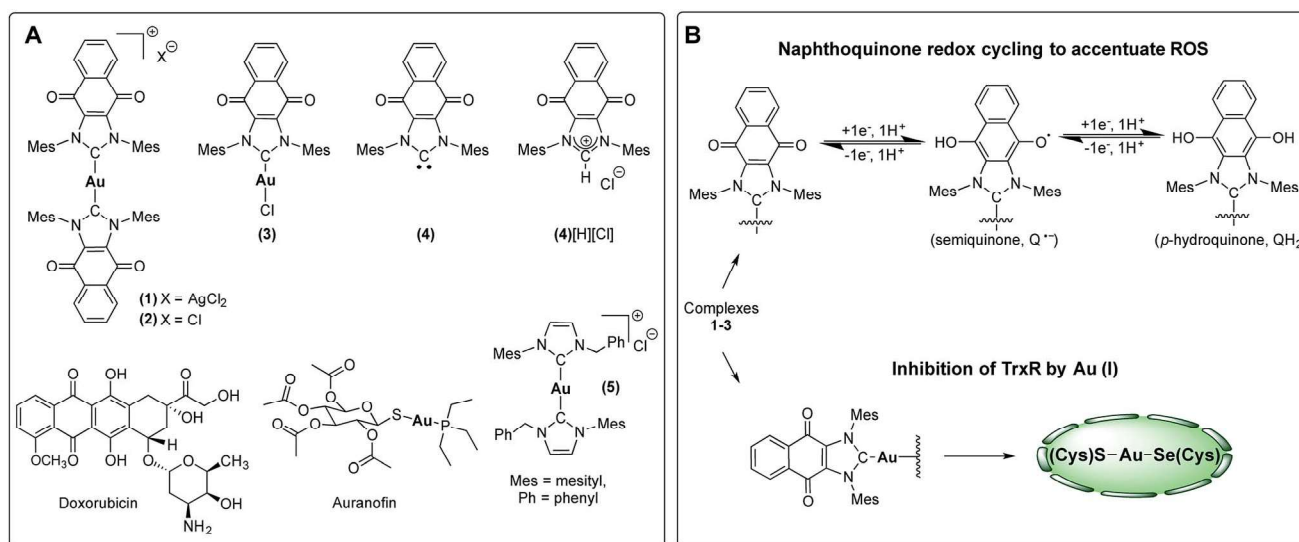
Fig. 3 (A) Complexes studied and (B) proposed dual mechanism of action for naphthoquinone functionalized gold(I) complexes [NHC–Au–NHC][X] (X = Cl − or AgCl 2 − , 1–3).
