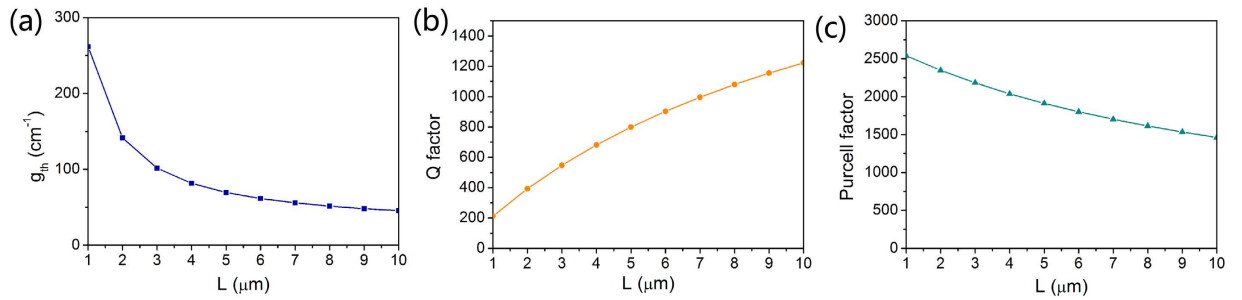
Figure 6. Lasing properties with varying cavity length. Dependences of (a) g_m , (b) quality factor Q and (c) Purcell factor on L .
