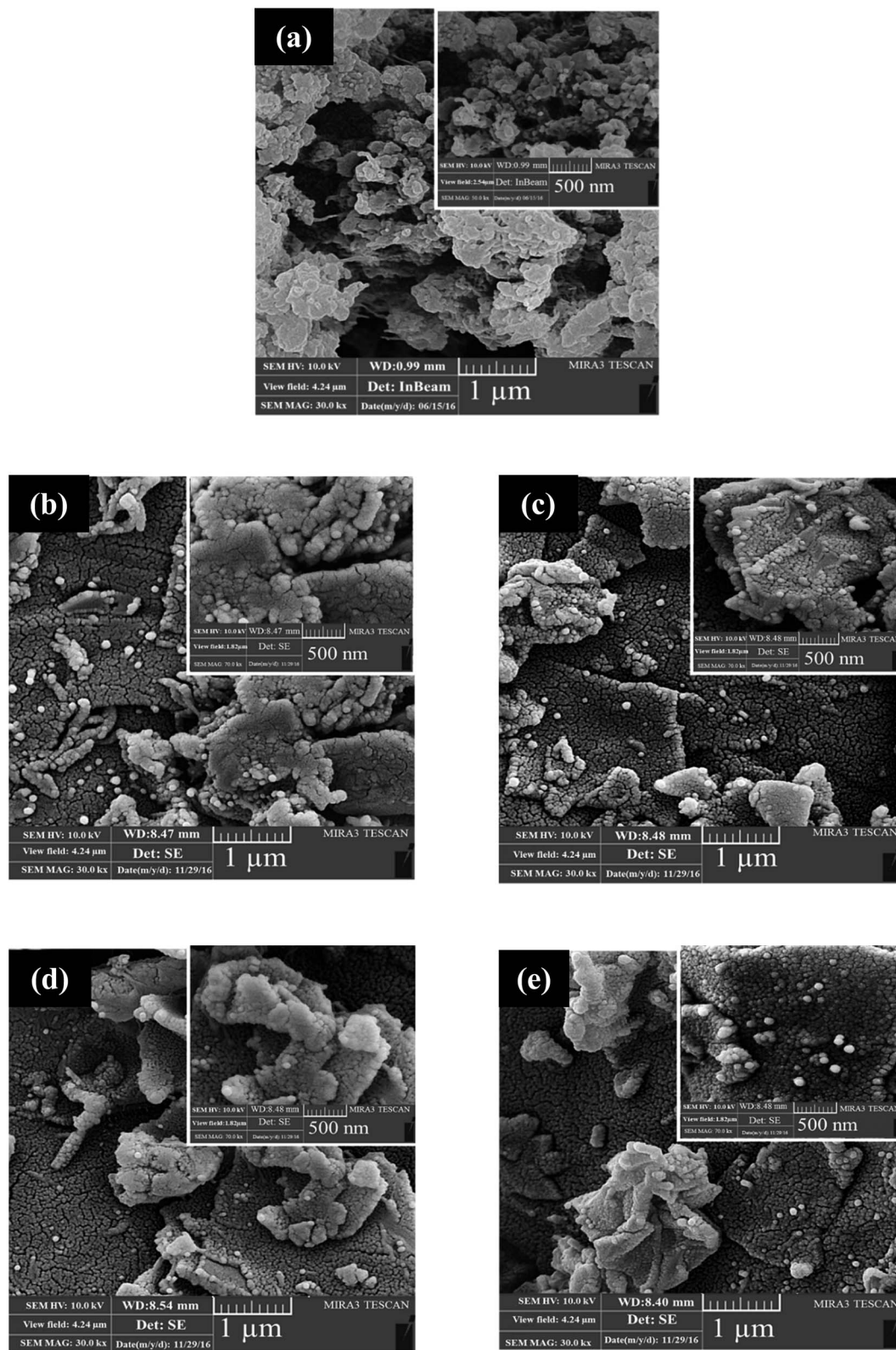
Fig. 4 FESEM images of (a) PANI, (b) PANI-PGO (0.05), (c) PANI-PGO (0.1), (d) PANI-PGO (0.2), and (e) PANI-PGO (0.4).
