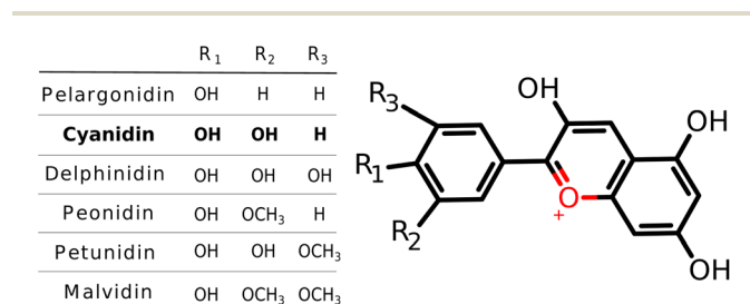
Scheme 1 The molecular structure of the six most common anthocyanidin dyes.
