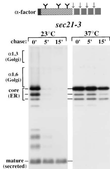
Figure 2. \alpha -factor processing and maturation in sec21-3 . \alpha -factor is schematized at the top, showing the signal sequence (black), pro segment (hatched lines), three N-linked glycosylation sites (Y), and late Golgi cleavage sites (white arrows) which generate the four mature peptides. sec21-3 (EGY1213) cells were incubated for 5 min at 23 or 37°C, pulse-labeled for 10 min with Tran 35 S, then chased for 15 min. Equal numbers of cells were removed at indicated timepoints. \alpha -factor was recovered by immunoprecipitation and visualized by SDS-PAGE and fluorography. The positions of core (ER)-, \alpha 1,6 manose (Golgi)-, and \alpha 1,3 manose (Golgi)-modified forms are indicated, as is the position of the mature, secreted peptide.
