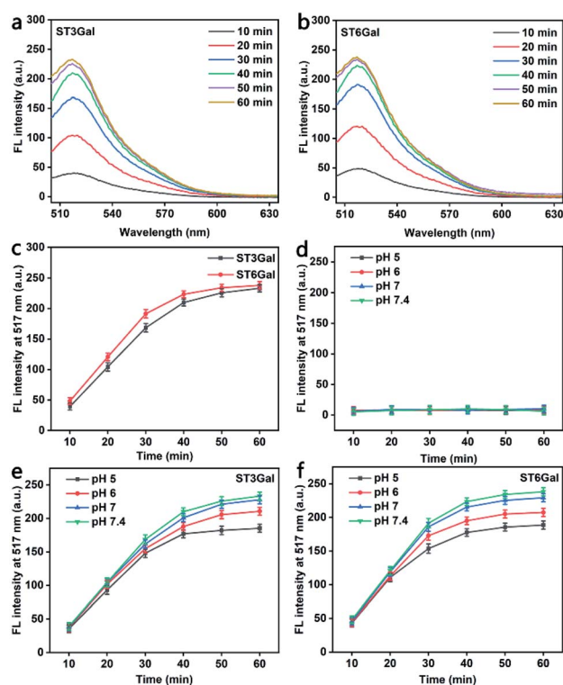
Fig. 2 In vitro response of MFMSNs. (a and b) Fluorescence spectra of 10 nM MFMSNs incubated with 5 μM of ST3Gal (a) or 100 μM of ST6Gal (b) and 100 μM of CMP-Sia in PBS (pH 7.4) for 10–60 min. (c) Corresponding time-dependent fluorescence intensity curves. (d–f) Time-dependent fluorescence intensity curves of 10 nM MFMSNs only (d), 10 nM MFMSNs with ST3Gal (e) or ST6Gal (f) and 100 μM of CMP-Sia at pH 5, 6, 7 and 7.4. Error bars represent \pm S.D. ( n = 3 ).
