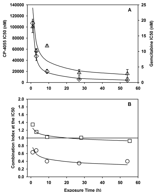
Figure 7. Effect of exposure time on the interaction of CP-4055 plus gemcitabine. Panel A: IC50 versus exposure time in HL-60 cells is shown for CP-4055 (diamonds) and gemcitabine (triangles) as single agents. Panel B: HL-60 (circles) or U937 (squares) cells were exposed simultaneously to CP-4055 in combination with gemcitabine at a fixed ratio of 1:0.0025 or 1:0.02, respectively. The combination index at the IC50 level of effect was then determined at each indicated time point. Bars: intra-assay standard error; lines: fit of data to the pharmacodynamic model C^n \times T = k .
