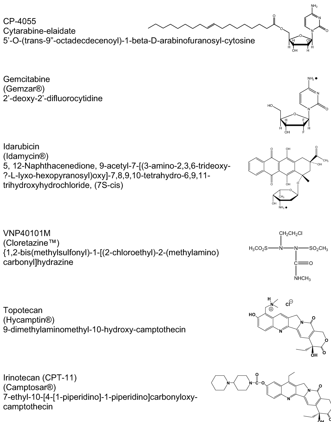
Figure 1. Structures of drugs under study.
