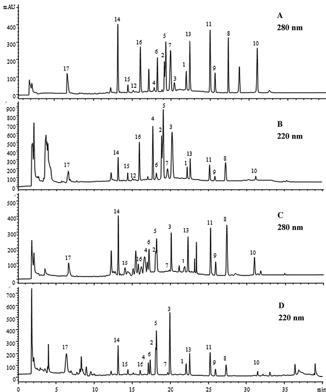
Figure 2 – High performance liquid chromatography of solution of standards (A) 280 nm and (B) 220 nm, and samples (C) at 280 nm and (D) 220 nm. Peaks: 1, rubescensin K; 2, oridonin; 3, ponigidin; 4, rosthorin; 5, enmenol; 6, nodifloretin; 7, pedaltin; 8, penduletin; 9, 5,8,4'-trihydroxy-6,7,3'-trimethoxyflavone; 10, 5,4'-dihydroxy-6,7,8,3'-tetramethoxyflavone; 11, cirsioliol; 12, quercetin; 13, luteolin; 14, caffeic acid; 15, isoacteoside; 16, rosmarinic acid; 17, methyl ursolate.
