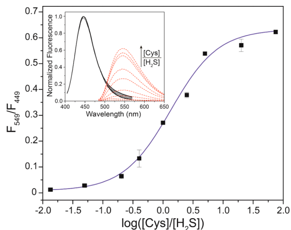
Figure 2. Ratiometric response ( F_{549}/F_{449} ) of NBD-Coum to varying Cys:H 2 S stoichiometries (75:1, 20:1, 5:1, 2.5:1, 1:1, 1:2.5, 1:5, 1:20, and 1:75). Inset: Resultant fluorescence spectra from varying Cys:H 2 S ratios. Normalized coumarin fluorescence ( \lambda_{\text{ex}} = 400 nm, \lambda_{\text{em}} = 449 nm) remains constant while NBD-Cys fluorescence ( \lambda_{\text{ex}} = 475 nm, \lambda_{\text{em}} = 549 nm) increases with [Cys]/[H 2 S]. Conditions: 5 \mu M NBD-Coum, 250 \mu M combined NaHS + Cys, PIPES buffer (50 mM, 100 mM KCl, pH 7.4). Data were acquired after 15 min incubation at 25 ^{\circ} C. Each data point represents the average of three trials. Error bars were calculated as standard error.
