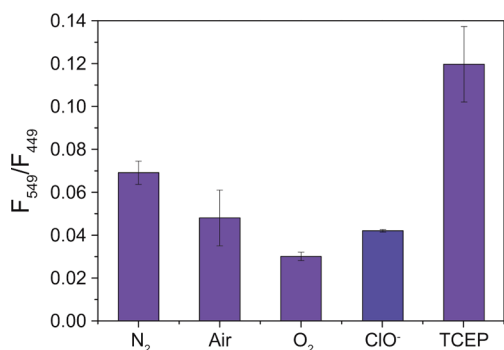
Figure 4. Response of the sulfur pool containing H 2 S, Cys, and cystine to oxidative and reductive influences. Relative Cys:H 2 S ratios decrease under oxidative conditions and increase under reducing conditions. Conditions: The initial sulfur pool (125 \mu M H 2 S, 125 \mu M Cys, 250 \mu M cystine) was incubated in PIPES buffer (50 mM, 100 mM KCl, pH 7.4) for 60 min at 25 ^{\circ}\text{C} under each redox condition and treated with 5 \mu M NBD-Coum.
