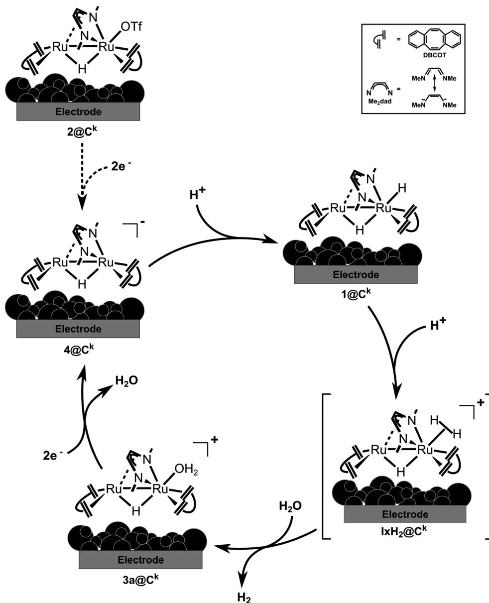
Fig. 10 Proposed mechanism for hydrogen evolution reaction by water electrolysis occurring onto the 2a@C^k cathode within the cell.
