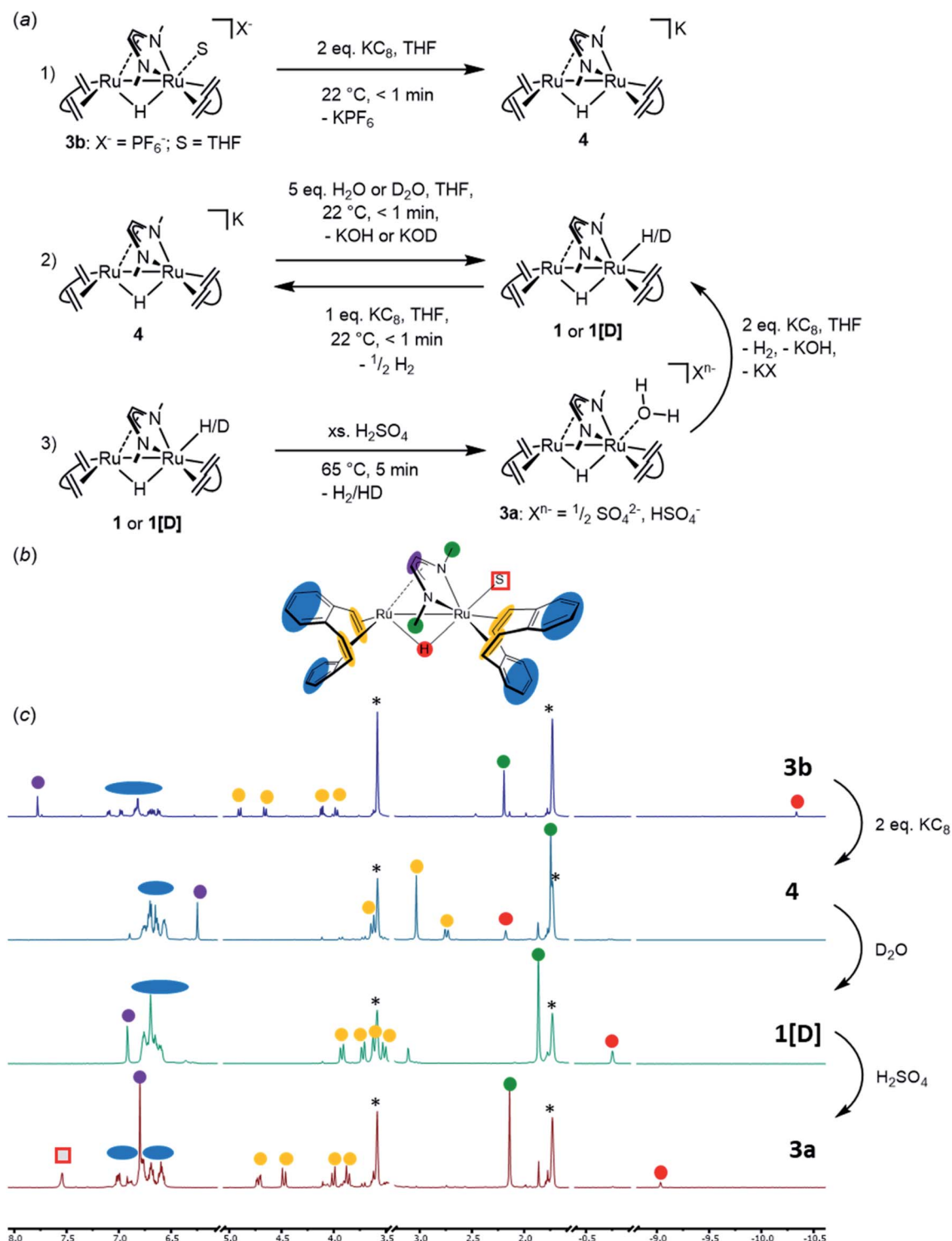
Fig. 8 (a) Schematic presentation of stoichiometric reactions (1), (2), (3) with complexes 3b , 4 , 1 (or 1[D] ), respectively. These were followed by in situ ^1H -NMR spectroscopy in THF[D_8] . (b) Structure of the generic complex [Ru_2(S)(\mu-H)(Me_2dad)(dbcot)_2] ( S = solvent molecule) with color coding for easier allocation of the ^1H -NMR signals. (c) Stack plot of ^1H NMR spectra taken after every indicated reactions (1) (top); (2) (middle); and (3) (bottom). The colored dots indicate the signals of the corresponding color coded protons in the formula given in (b). The red square marks the signal of the coordinated water in complex 3a . Note that D_2O was chosen in the 2nd transformation to yield complex 1[D] with a deuterium in terminal position. See Fig. S12† for a comparison of the spectra of 1 and 1[D] .
