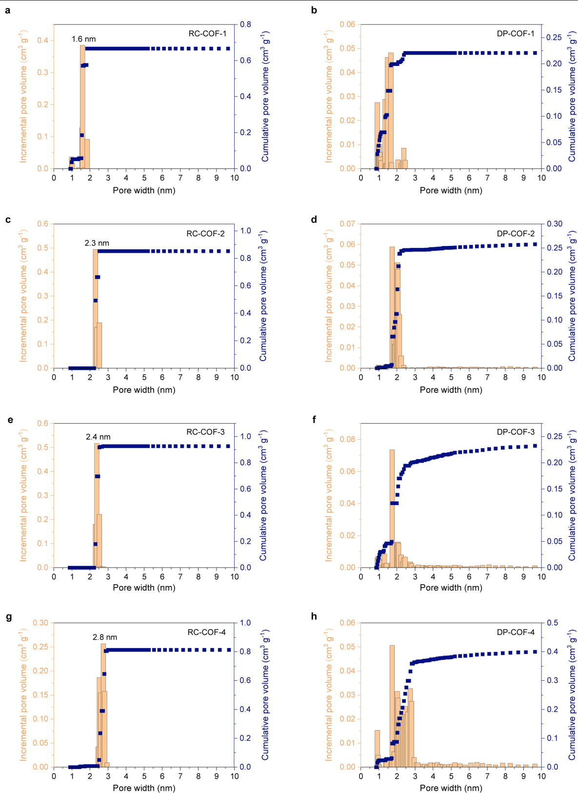
Extended Data Fig. 3 | Pore size distributions. a–h, Pore size distribution profiles for RC-COFs (a, c, e, g) and DP-COFs (b, d, f, h). The reconstructed COFs showed a much narrower pore size distribution, which reflected their enhanced crystallinity.
