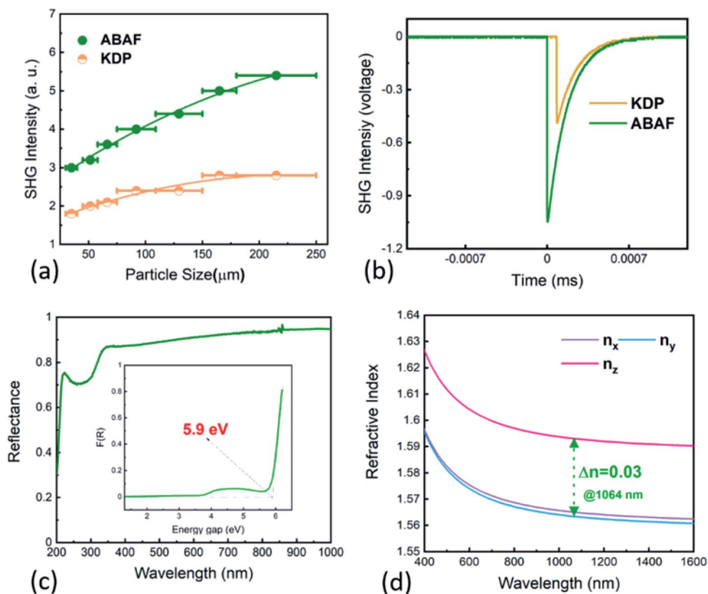
Fig. 2 Nonlinear and linear optical properties of ABAF. (a) Particle size dependent SHG test. (b) SHG signal traces of the oscilloscope. (c) The UV-Vis-NIR reflectance spectrum. (d) Calculated refractive index.
