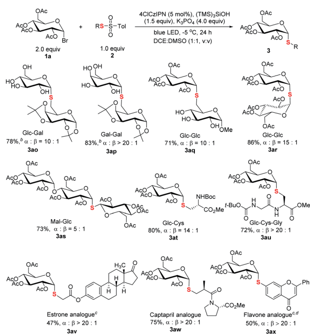
Scheme 5 Thiodiversification of pharmaceutically relevant structures. a Reaction conditions: unless specified, see footnote a of Table 1 and the ESI; † isolated yield; ratio of α and β anomers determined by crude 1 H NMR. b The product after hydrolysis. c Methylthiosulfonate used. d DCE : H 2 O (1.5 mL, 2 : 1, v/v) used as the solvent.
