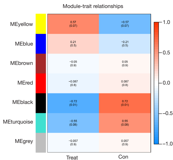
Figure 1 Correlation between the gene module and clinical traits of neuropathic pain-induced depression. The number above represents the correlation coefficient in the square, and the number in brackets represents the P value. Con, control; ME, module eigengene.
