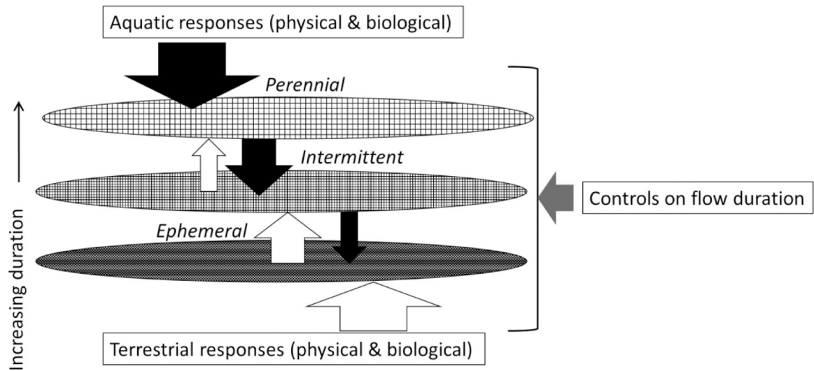
Figure 2. Conceptual figure illustrating indicators of streamflow duration. Response indicators are “filtered” along the gradient of streamflow duration, such that the strength of aquatic signal (black arrows; e.g., stream biota, fluvial geomorphology) declines and terrestrial signal (white arrows; e.g., terrestrial biota, soil development) increases with decreasing flow duration. Control indicators (gray arrow) are factors that govern streamflow duration from reach to landscape scales (e.g., meteorology, geology, land cover).
