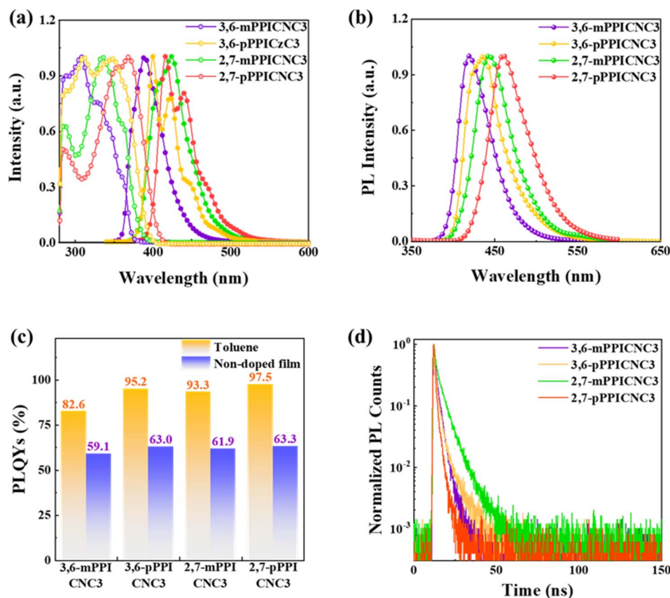
Fig. 3 (a) Normalized absorption and PL spectra of 3,6-mPPICNC3, 3,6-pPPICzC3, 2,7-mPPICNC3 and 2,7-pPPICNC3 in toluene solution ( 10^{-5} M). (b) Normalized PL spectra in the neat film. (c) PLQYs in toluene and the neat film. (d) Transient PL decay spectra in the neat film.
