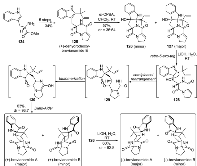
Scheme 24 Asymmetric total synthesis of brevipanamide A and B.
