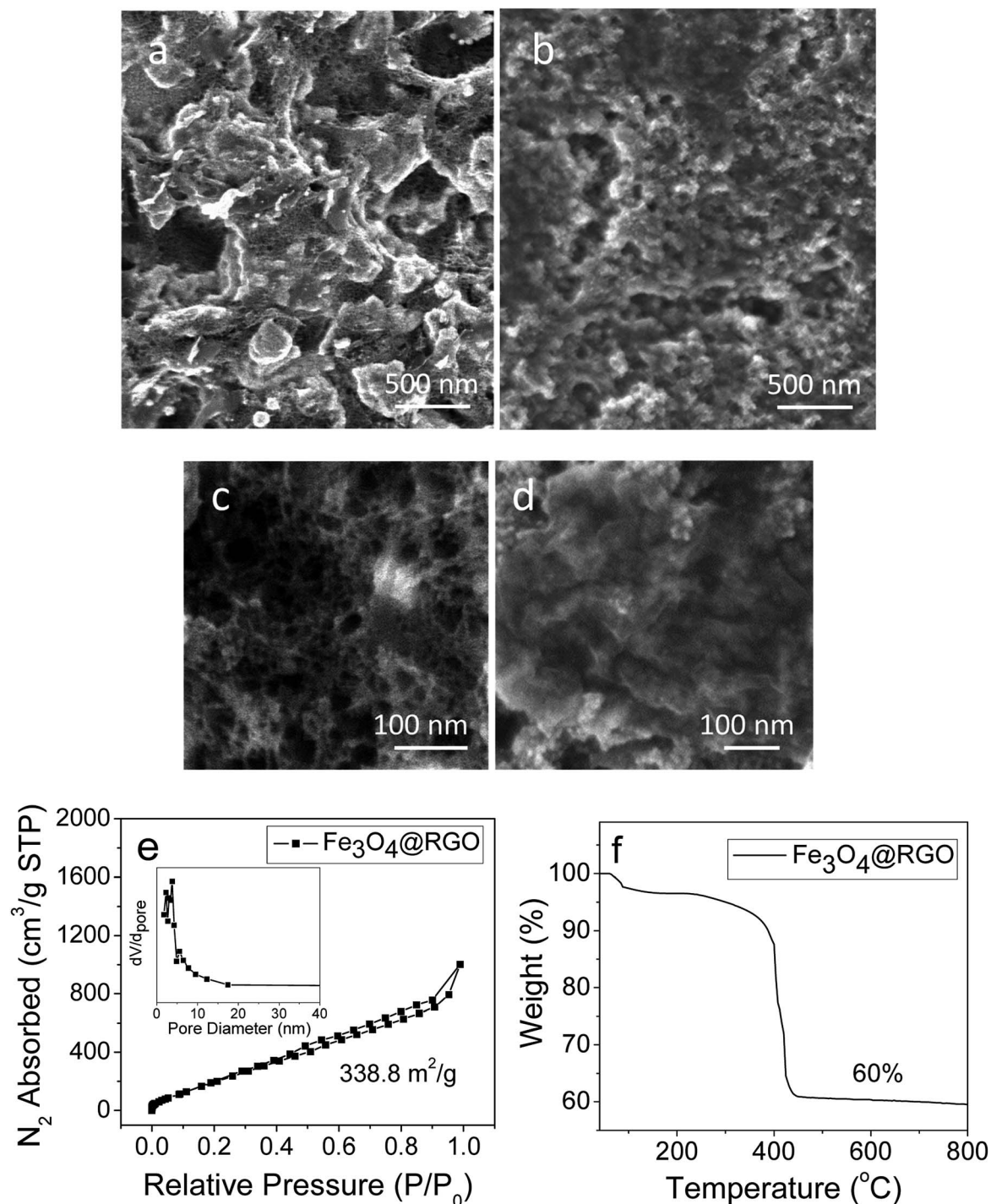
Fig. 7 (a and b) SEM images of PMAA-induced porous Fe 3 O 4 @RGO. (c and d) Citric acid-assisted stacked Fe 3 O 4 @RGO. (e) Nitrogen adsorption-desorption isotherms and pore-size distribution of PMAA-induced porous Fe 3 O 4 @RGO (inset figure). (f) TGA curve of Fe 3 O 4 @RGO acquired with a temperature ramp of 5 °C min -1 in air.
