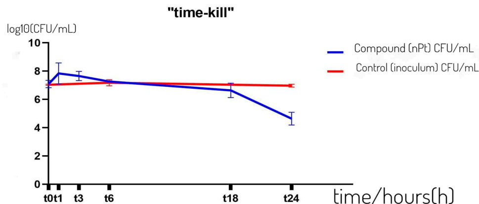
Figure 1. Number of colonies of Klebsiella pneumoniae ESBL+ MFBF 10690 over time (h) treated with nPt ( c = 2 \times \text{MIC} ) relative to the control. CFU—colony forming unit; t—time.
