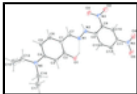
Fig. 1. Molecular view of I with the atom labeling scheme. Displacement ellipsoids are drawn at the 30% probability level. Only the major component of the disordered ethyl group is shown. H atoms are represented as small spheres of arbitrary radii. Intramolecular H bond is shown as dashed line.
