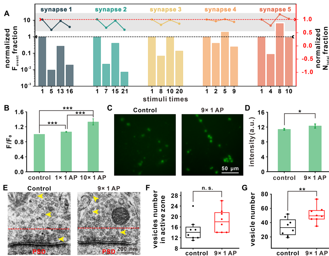
Fig. 3 The variation in the neuronal vesicle amount after repetitive stimuli. (A) Normalized histograms of F_{event} under representative stimuli times (first one, the stimulus with minimum F_{event} before recovery, the stimulus with maximum F_{event} during recovery, and the last one with detected exocytotic events) compared with the event amount of the same synapse ( n = 5 ) in the first stimulus, and normalized line graphs of N_{total} under different stimuli times compared with the release number of the same synapse in the first stimulus. (B) Normalized fluorescence statistical analysis of the same DAergic neuron ( n = 72 ) showing the change in the intracellular Ca^{2+} concentration revealed by Fluo-4 AM before or after the first and 10th EFS; mean \pm SD, ***p \leq 0.001 . (C) Representative microscopic images of DAergic neurons without EFS or with 9 stimuli labeled with synaptophysin (SV marker, green), and the (D) corresponding statistical analysis; mean \pm SD, *p \leq 0.05 . (E) TEM images of SVs (marked by yellow arrows) in the VTA presynaptic terminal from 7 days SD rat brain slices without EFS or with 9 stimuli (PSD: post synaptic density), and the corresponding statistical analysis of the vesicle number in the active zone (the area between the red dashed line and the presynaptic membrane) (F), and in the (G) total presynaptic structure; n_{cell} = 8 in each group, n.s.: no significance, **p \leq 0.01 .
