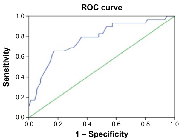
Figure 2 ROC curve for V_{25} . Abbreviation: ROC, receiver operating characteristic.
