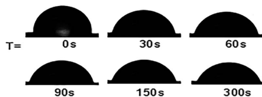
Fig. 8 Droplet shape during wetting.
