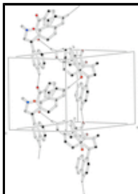
Fig. 2. Molecular packing of the title compound, viewed along the a axis; H-bonds are shown as dashed lines. For the sake of clarity, H atoms, not involved in hydrogen bonds, have been omitted
