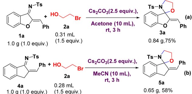
Scheme 6 Gram-scale synthesis.
