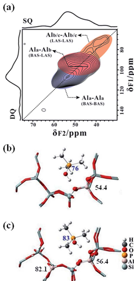
Fig. 6 2D ^{27}\text{Al} - ^{27}\text{Al} DQ-SQ MAS NMR spectrum (a) of dehydrated and TMPO-loaded H-ZSM-5 zeolite (P/Al = 0.42), recorded at 18.8 T with a spinning speed of 20 kHz. Local theoretically optimized structures of TMPO adsorbed at the isolated Brønsted site (b) and the Brønsted/Lewis acid synergetic site (c) with a tri-coordinated FAL in close proximity. The predicted ^{31}\text{P} chemical shifts of the TMPO (blue numbers) and ^{27}\text{Al} chemical shifts of the corresponding acid sites (black numbers) are labeled in ppm.
