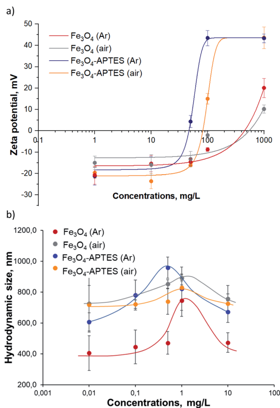
Fig. 3 (a) Zeta-potential and (b) hydrodynamic diameter of aqueous suspensions of MNPs: a dose-effect study (ultrasonication 10 min, dilution in water).
