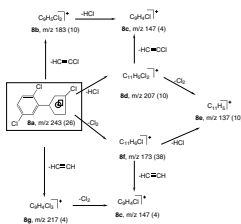
Scheme 3: Principal EI-MS fragmentation pathways of phenylcyclopentadienyl cation 8a ( m/z 243) formed from 2',3,5'-trichlorobiphenyl-4-yl ester 2,2,2-trichloroethyl ester 8 . The fragmentation pattern resulting in the formation of 8a from the corresponding molecular ion is analogous to the pathways shown in Scheme 1.
