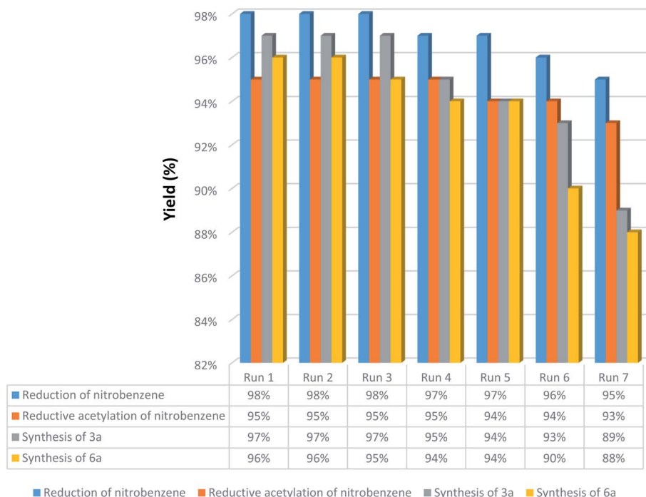
Fig. 11 Recoverability and reusability experiments of the dendritic \text{Fe}_3\text{O}_4@\text{SiO}_2@\text{KCC-1}@MPTMS@Cu^{II} mesoporous nanocomposite.
