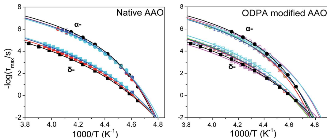
Fig. 7 Temperature dependence of \alpha and \delta -relaxation times in bulk E7 and E7 located within native AAO (left) and ODPa modified AAO (right). Both exhibit a VFT dependence and, most notably, reduction of T_g(\alpha) and T_g(\delta) with decreasing pore diameter. Varying diameters are depicted as follows, (black) bulk E7; (red) 400 nm; (green) 200 nm; (blue) 65 nm; (magenta) 35 nm; (cyan) 25 nm.
