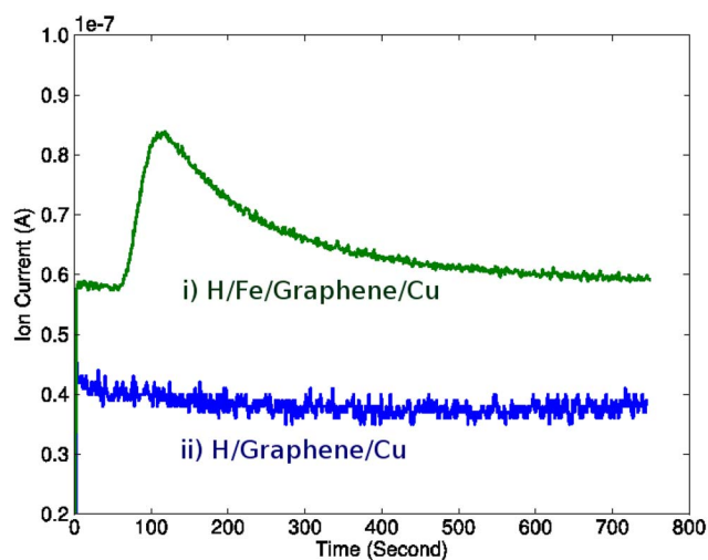
Figure 3 | Dehydrogenation as characterized by mass spectrometry where it is set to detect only hydrogen gas. Dehydrogenation was performed at 400^\circ\text{C} . i) Hydrogenated Fe on graphene/Cu and ii) hydrogenated graphene/Cu.
