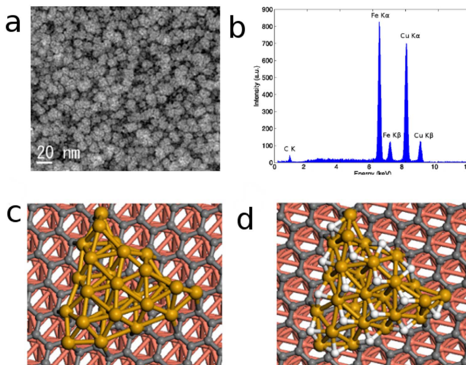
Figure 2 | (a) STEM images of Fe nanoparticles on graphene/Cu and (b) corresponding EDS analysis. Calculated atomic models of (c) \text{Fe}_{25} graphene/Cu(111) and (d) \text{Fe}_{25}\text{H}_{16} on graphene/Cu(111). Atomic color codes: Fe, ochre; H, white; C, gray; Cu, red.
