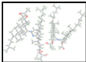
Fig. 1. The asymmetric unit of the title compound showing 30% probability displacement ellipsoids for non-H atoms. Both major and minor components of disorder are shown.
