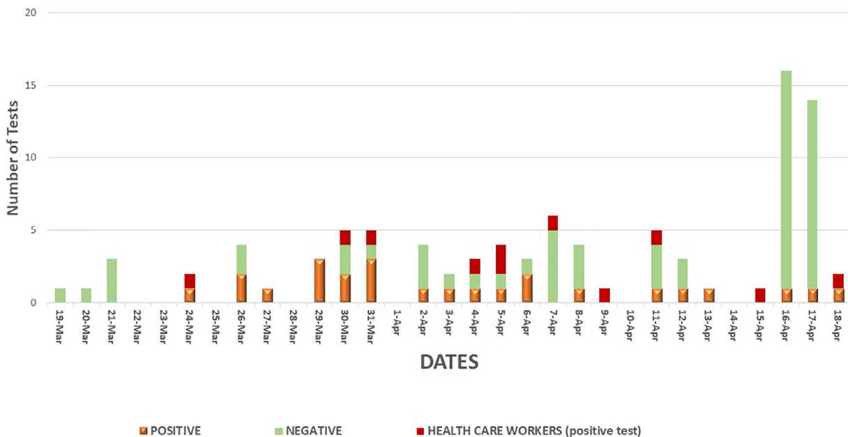
Fig 1. SARS-CoV-2 outbreak dates of tests.
