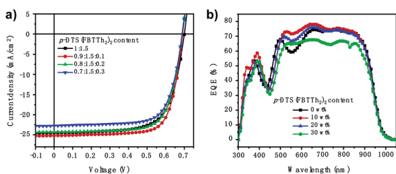
Fig. 2 (a) The J - V curves of PSCs with different p -DTS(FBTTh 2 ) 2 content levels. (b) The EQE spectra of the corresponding PSCs (calculated integrated current densities: 23.57 mA cm -2 , 24.46 mA cm -2 , 23.76 mA cm -2 , and 21.6 mA cm -2 ).
