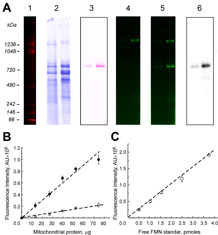
Fig. 3. Identification of Complex I FMN and FAD of \alpha KGDHC in DDM-solubilized brain and heart mitochondria. (A) Intact mitochondria were solubilized using a DDM/protein ratio of 3.6 g/g. Identical aliquots of 15 \mu g of total mitochondrial protein were loaded on an acrylamide gradient gel (3–12%). Heart (right) and brain (left) mitochondria samples were applied on the same gel and hrCN electrophoresis was performed as in Ref. [38]. Lanes 2, Coomassie stained gel strips showing the presence of complexes (I–V) with molecular weight markers (Lane 1); Lanes 3, complex I in gel activity strips; Lanes 4 and 5, flavin fluorescence from the same strip before (4) and after (5) treatment with 20% SDS (Excitation/Emission = 473/530 nm). Lanes 6, complex I immunodetection by Western blot using antibody against NDUFS8 subunit; (B) dependence of the flavin fluorescence intensity in the complex I (black circles) and \alpha KGDHC (grey circles) bands upon protein load on the gel. Values are mean \pm SEM, n = 4; (C) calibration curve for flavin fluorescence signal made of standard free FMN solution applied directly on a gel and intensity of fluorescent spots measured (mean \pm SEM, n = 3).
